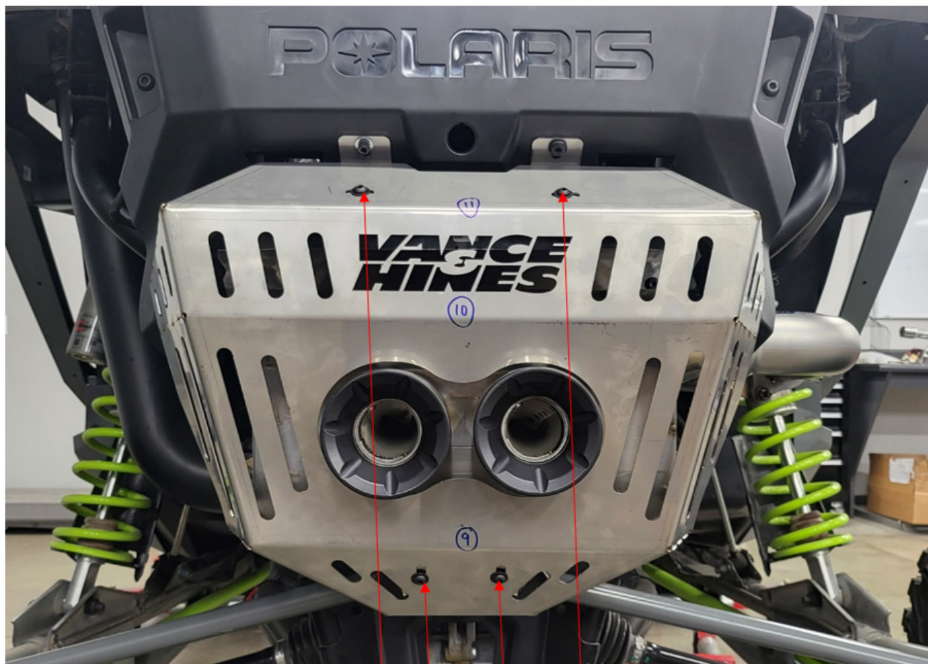
FIG 8: REAR COVER ALIGNMENT
