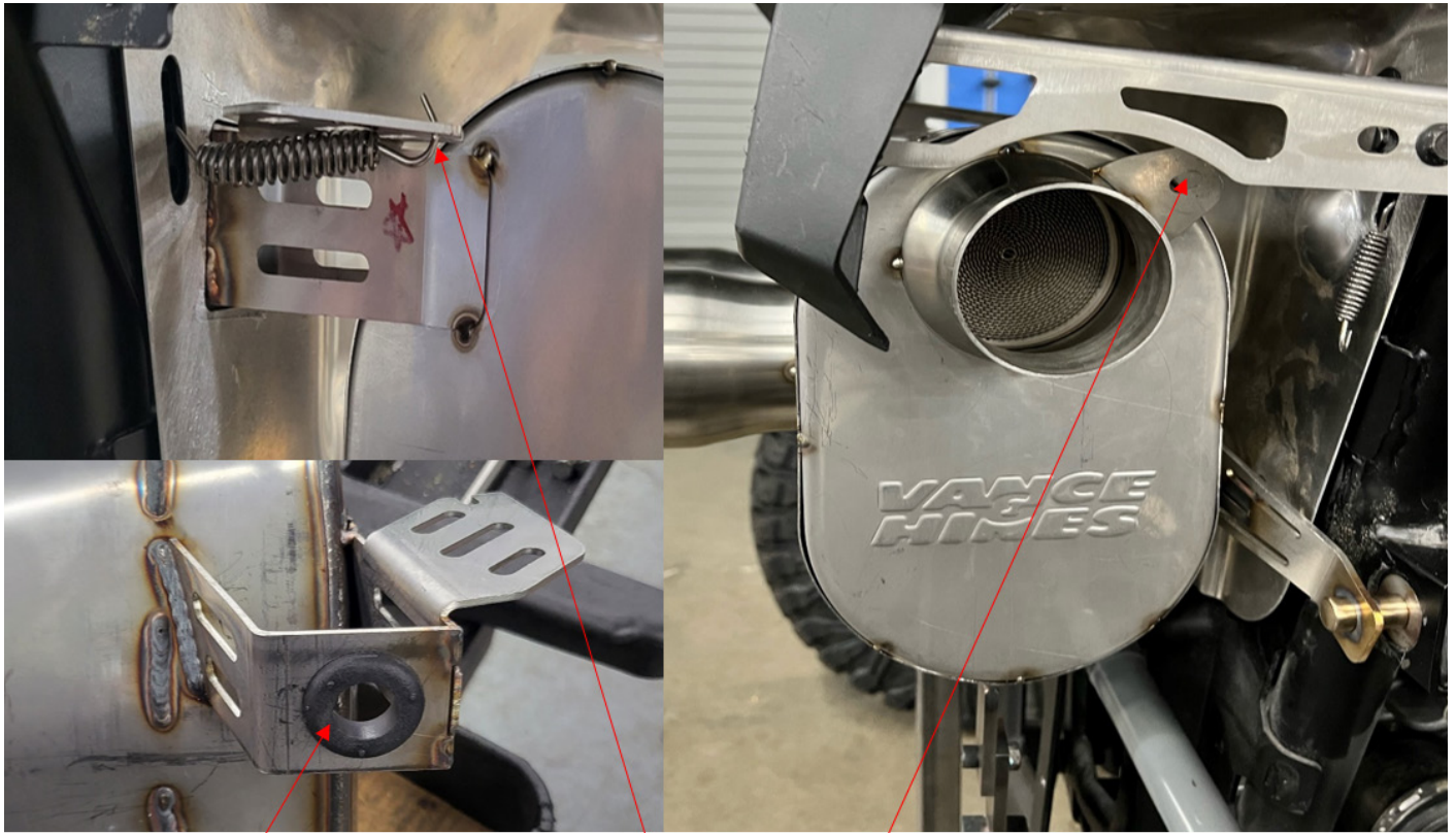
FIG 5: V&H EXHAUST SPRING MOUNT LOCATION
